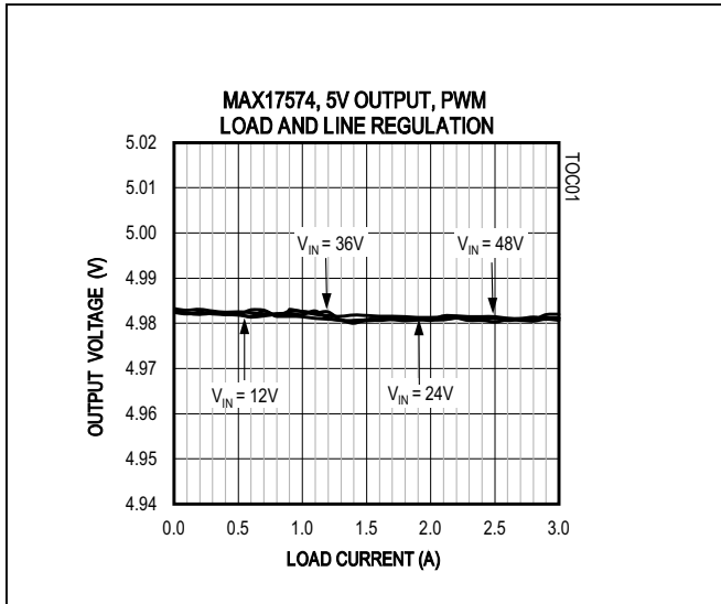
Figure 1. MAX17574 5V Output Load and Line Regulation (PWM Mode)
