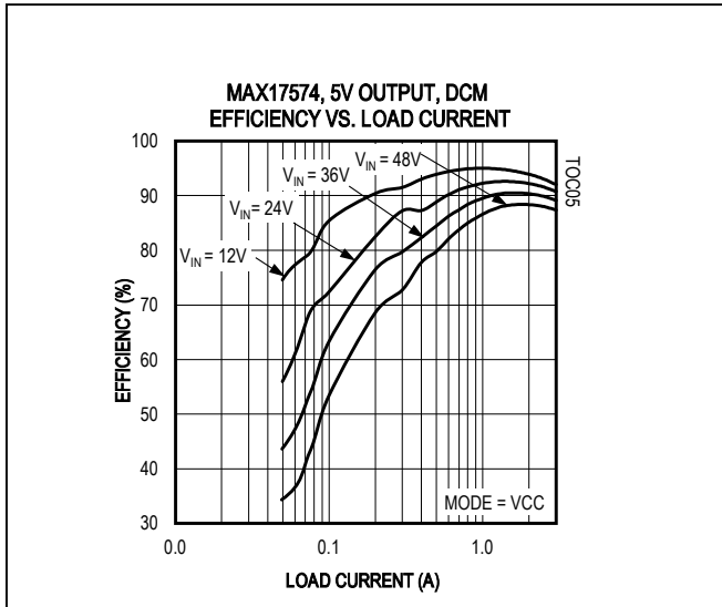
Figure 5. MAX17574 5V Output Efficiency (DCM Mode)
