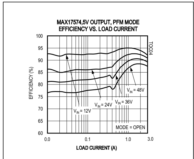
Figure 4. MAX17574 5V Output Efficiency (PFM Mode)
