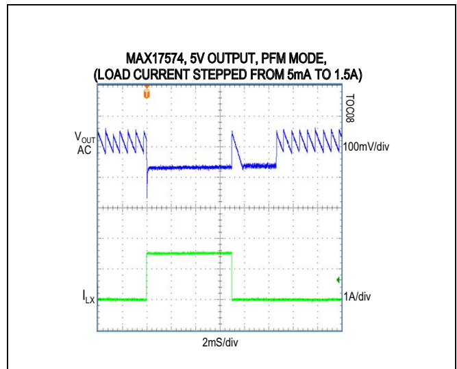
Figure 8. MAX17574 5V Output, 5mA to 1A Load Transient (PFM Mode)
