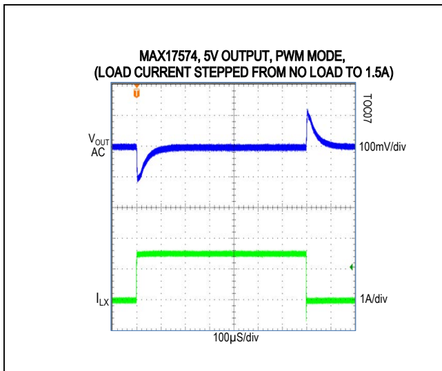
Figure 7. MAX17574 5V Output, No Load to 1A Load Transient (PWM Mode)
