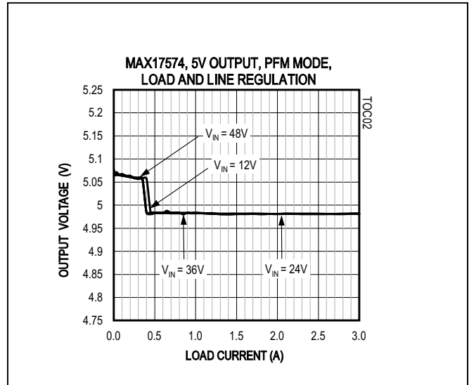
Figure 3. MAX17574 5V Output Load and Line Regulation (PFM Mode)
