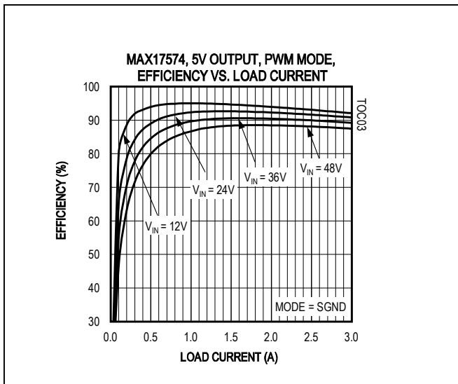
Figure 2. MAX17574 5V Output Efficiency (PWM Mode)
