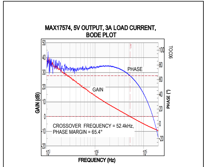
Figure 6. MAX17574 5V Output Full Load Bode Plot ( V_{IN} = 24V )
