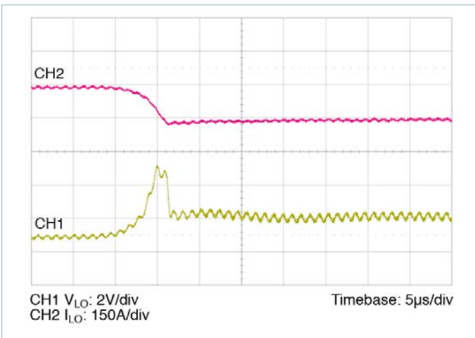
Figure 16 — 150A – 0A transient response: C_{HI\_IN\_EXT} = 300\mu\text{F} , no external C_{LO\_OUT\_EXT}
