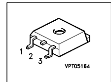
PG-TO263
