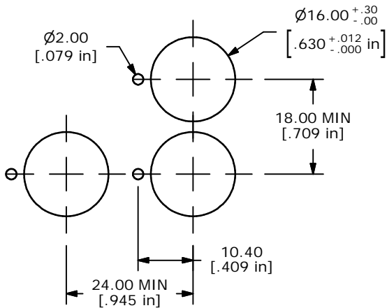
PANEL MOUNTING
