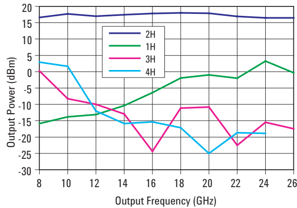
Figure 1. Output Power vs. Output Freq. @ Pin=+3dBm
