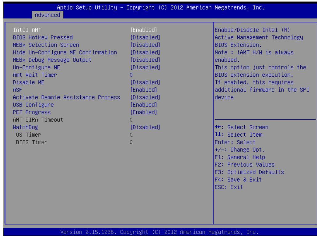
Figure 3.10 AMT Configuration
