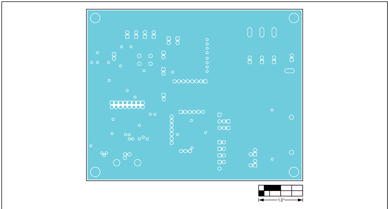
Figure 13. MAX9271 Coax EV Kit PCB Layout—Ground Layer 2
