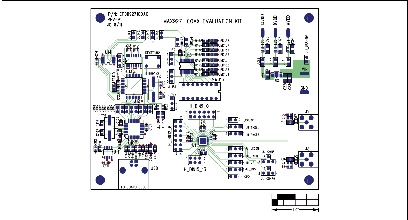
Figure 12. MAX9271 Coax EV Kit PCB Layout—Component Side
