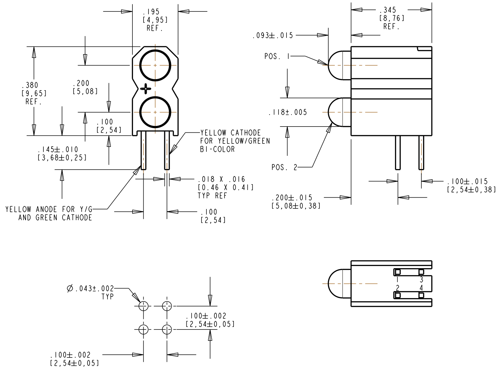
RECOMMENDED HOLE PATTERN GAUGE
