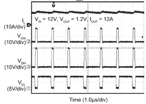
MIC2101 Switching Waveforms ( I_{OUT} = 12A )
