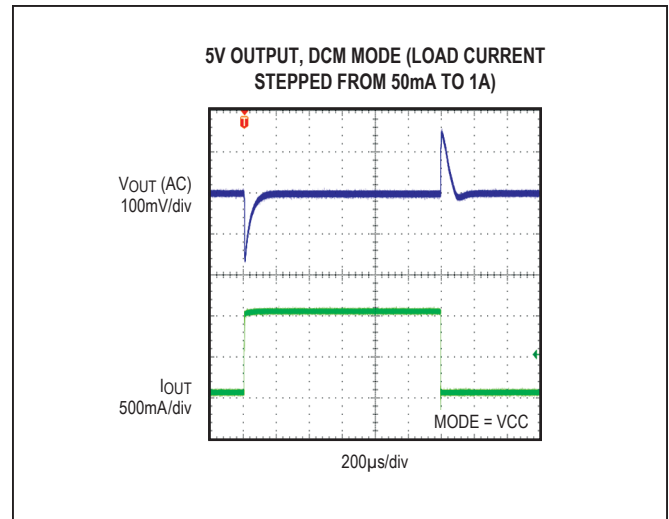
Figure 9. MAX17543 5V Output, 50mA to 1A Load Transient (DCM Mode)
