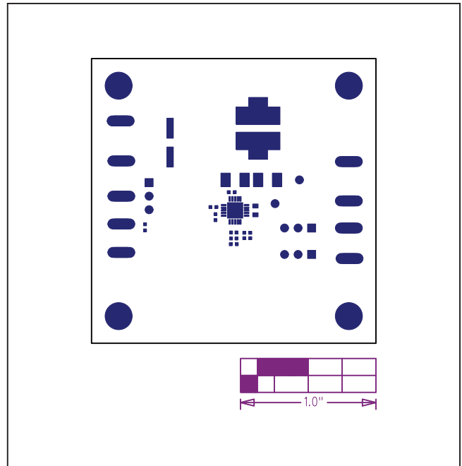
Figure 17. MAX17543 5V Output EV Kit Component Placement Guide—Top Solder Mask
