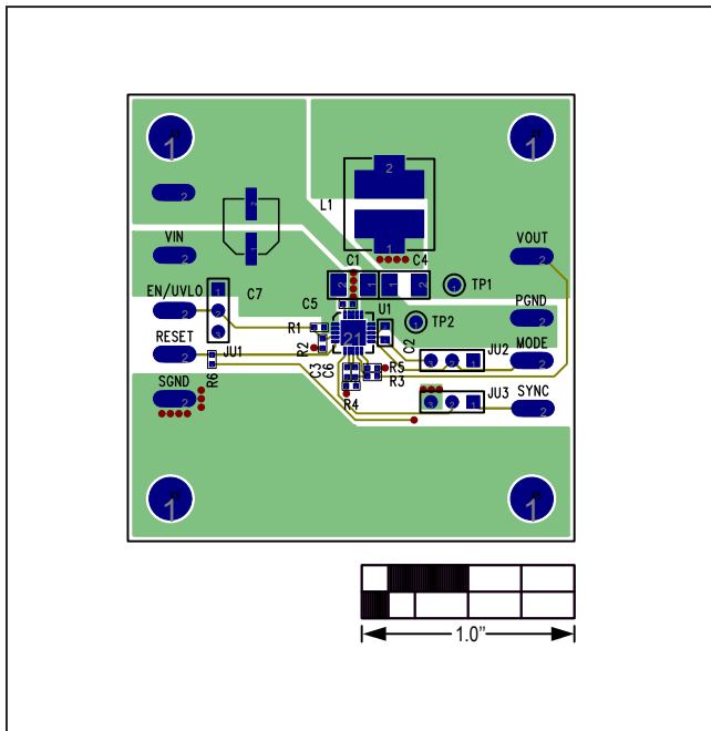
Figure 13. MAX17543 5V Output EV Kit Component Side PCB layout
