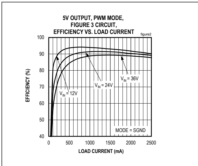
Figure 2. MAX17543 5V Output Efficiency (PWM Mode)
