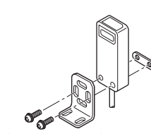
Sensor head mounting bracket for LA-305 MS-LA3-2 (Accessory) (Note)
