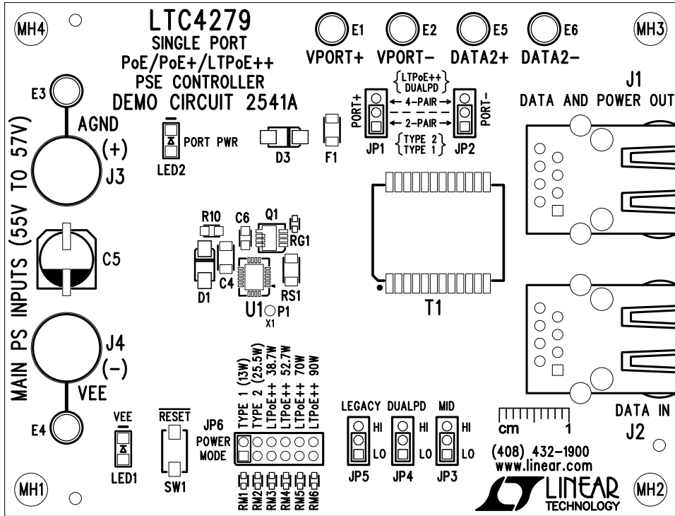
Top Assembly
