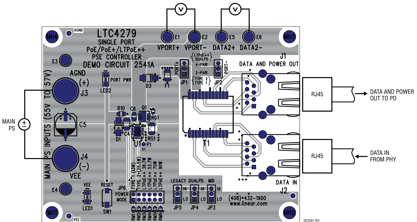
Figure 1. DC2541A Connection Diagram
