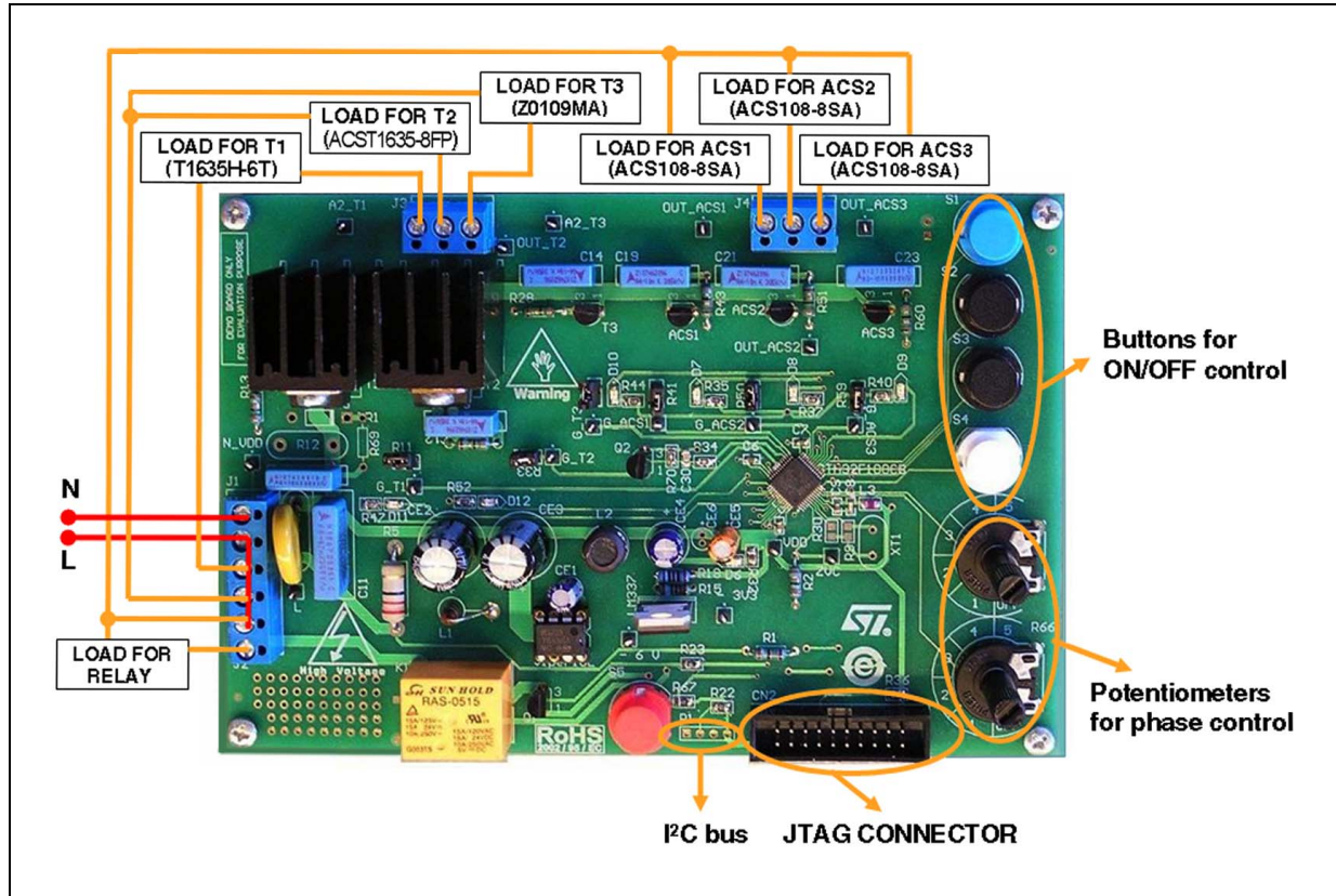
Figure 2. Board connector
