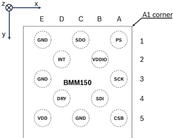
Pin configuration (top view)
