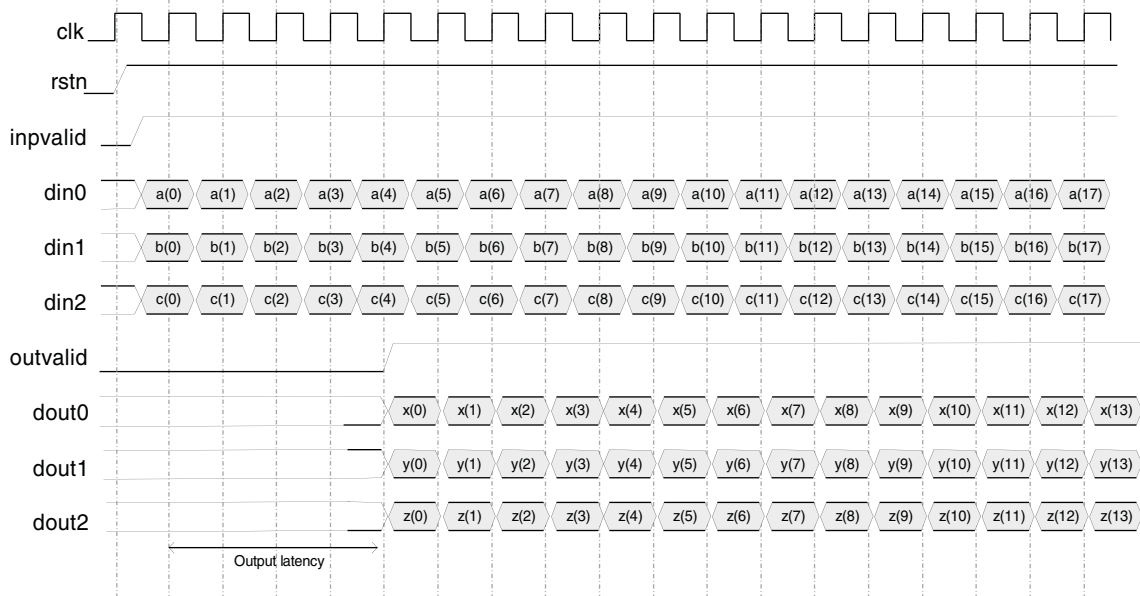
Figure 2-4. Parallel Architecture
