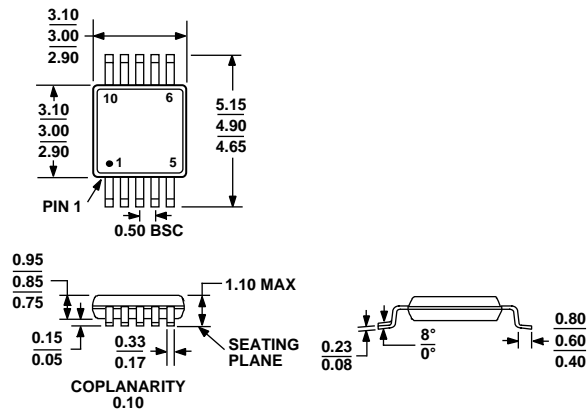
Figure 22. 10-Lead Mini Small Outline Package [MSOP] (RM-10) Dimensions shown in millimeters
