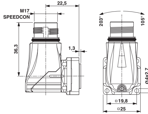
Dimensioned drawing
