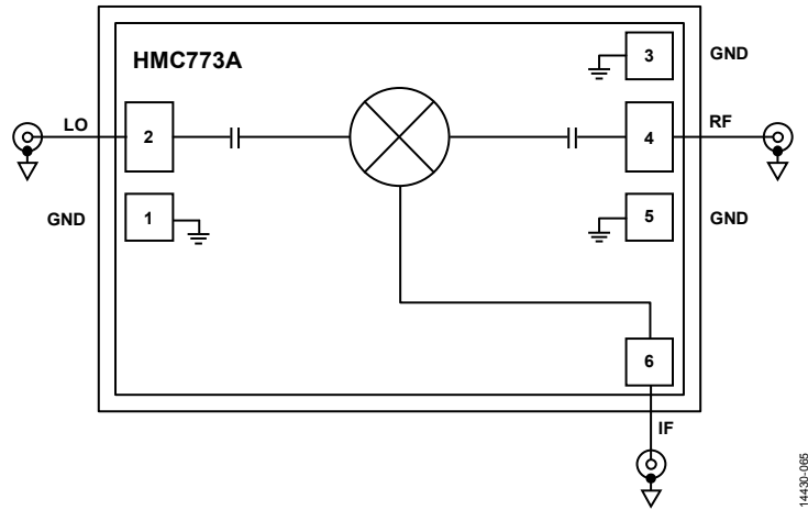
Figure 63. Typical Application Circuit
