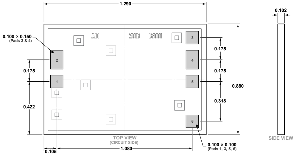
Figure 67. 6-Pad Bare Die [CHIP] (C-6-12) Dimensions shown in millimeter
