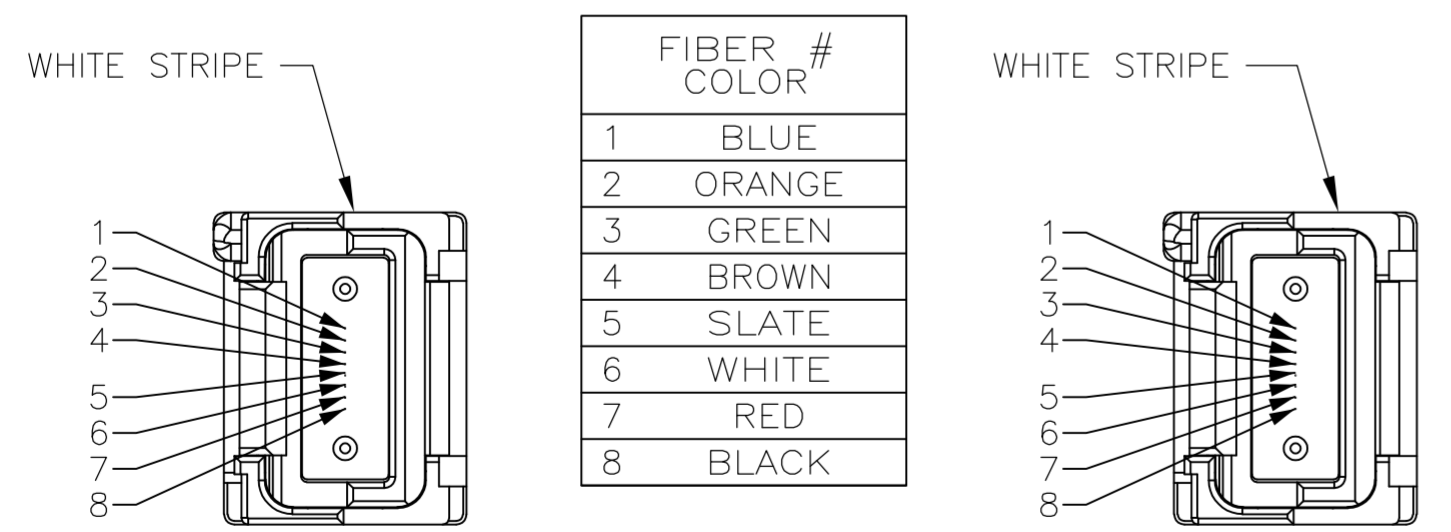
VIEW A-A VIEW B-B LIGHTRAY MPX CONNECTOR FIBER PATH
