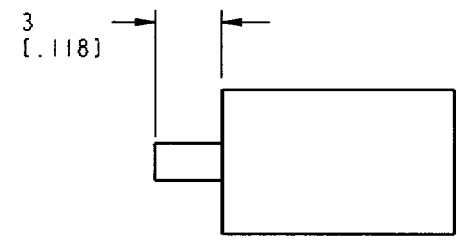
RECOMMENDED CABLE STRIPPING DIMENSIONS SCALE 3.000
