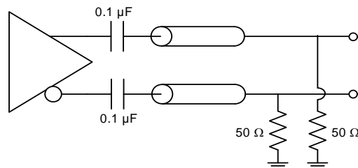
Figure 6. Alternative CML Output Buffer Connection
