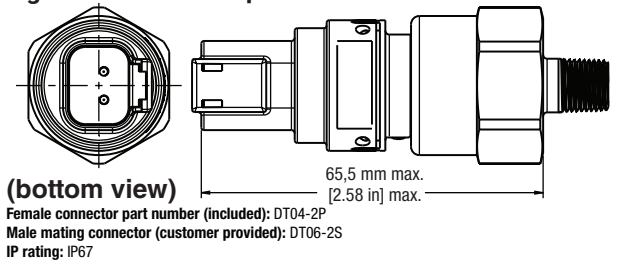
Figure 17. Wire out
