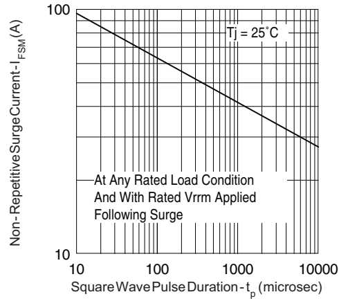
Fig. 6 - Maximum Peak Surge Forward Current vs. Pulse Duration
