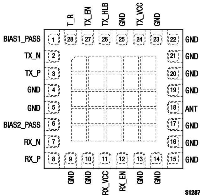
Figure 2. SKY65337-11 Pinout – 28-Pin MCM (Top View)
