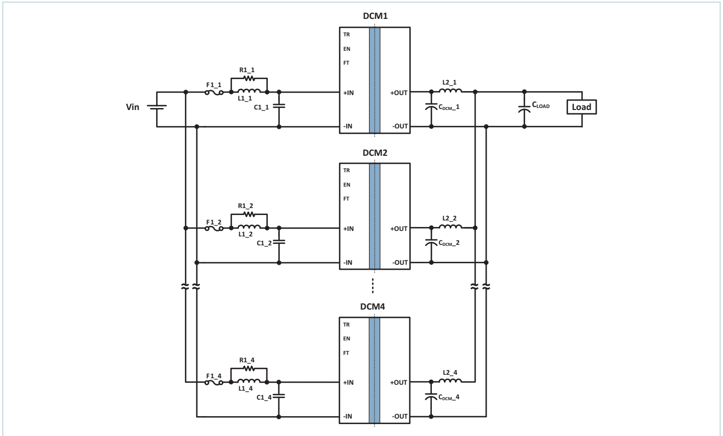
Typical Application 1: DCM300P120x400A40 in an array of four units
