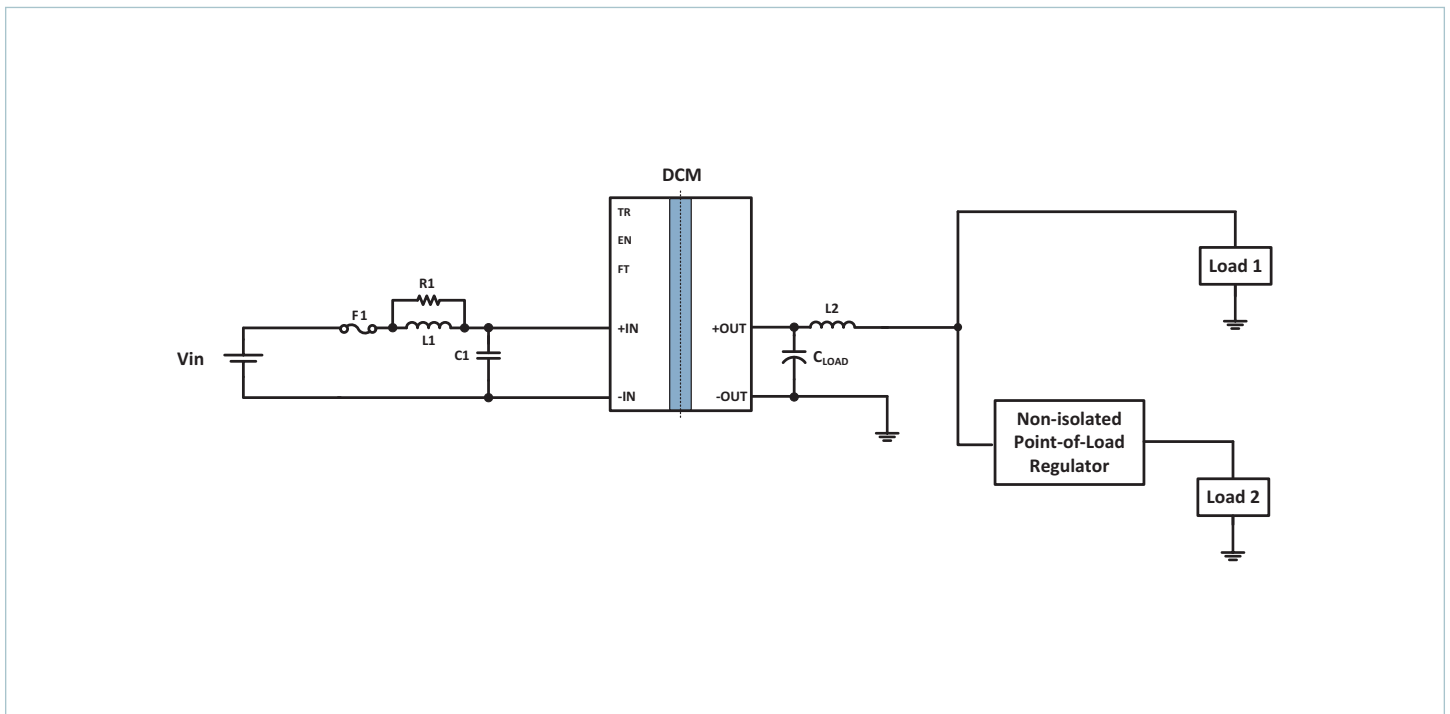
Typical Application 2: Single DCM300P120x400A40, to a non-isolated regulator, and direct to load
