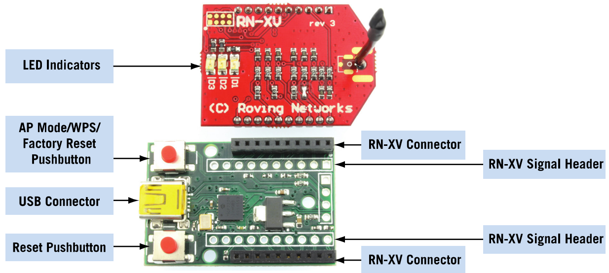
Figure 1. RN-XV-EK Components
