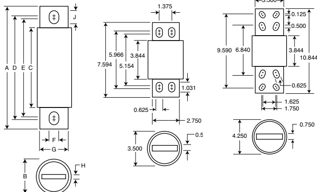
Fig. 1: 5-800A
