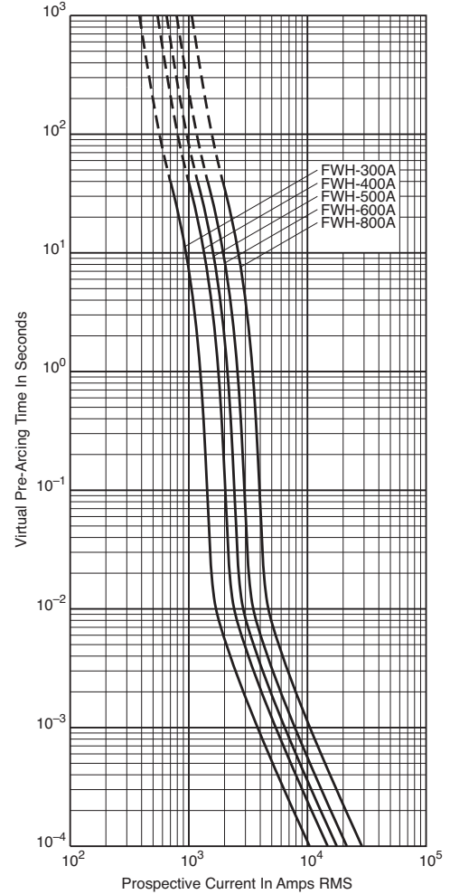
Time-Current Curve
