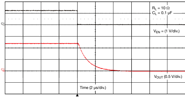
Fig. 21 - Turn-Off Time ( V_{IN} = 1.2 \text{ V} )
