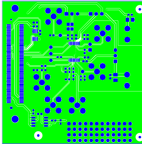
Figure 36. AD9832 Evaluation Board Component Side
