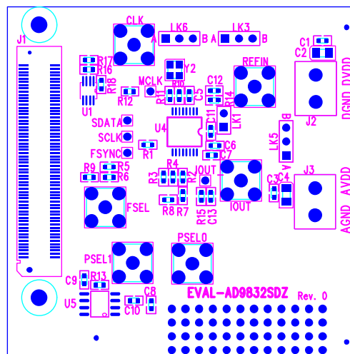
Figure 38. AD9832 Evaluation Board Solder Side
