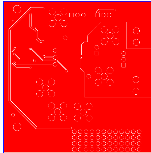
Figure 37. AD9832 Evaluation Board Silkscreen
