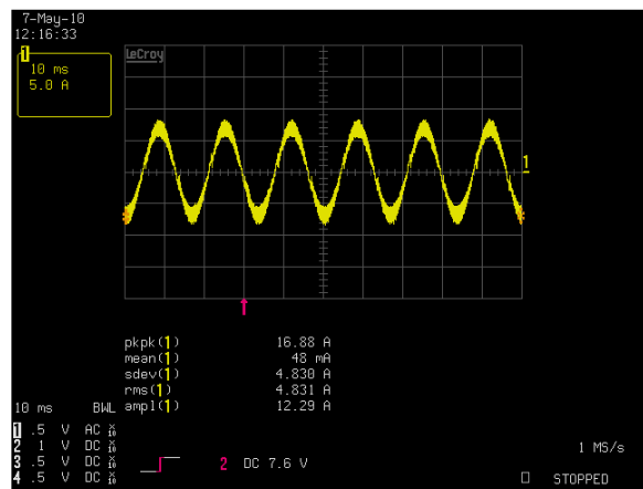
Figure 24: ADN20-24-1PM-C Input Current Waveform Vin = 115Vac Io = 20.0A Ch 1: I IN
