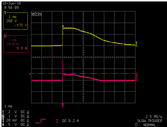
Figure 3: ADN5-24-1PM-C Inrush Current Vin = 230Vac Io = 0A, Turn on angle = 90 deg Ch 1: AC Mains Ch 2: Io
