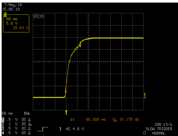
Figure 25: ADN20-24-1PM-C Output Voltage Startup Characteristic Vin = 90Vac Io = 20.0A, Output Capacitance = 330uF/A Ch 1: Vo
