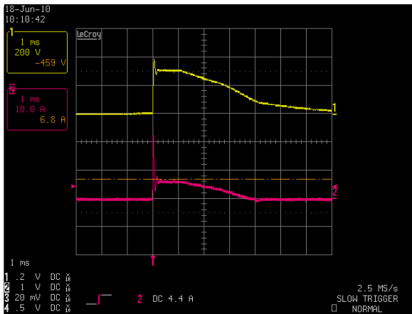
Figure 23: ADN20-24-1PM-C Inrush Current Vin = 230Vac Io = 0A, Turn on angle = 90 deg Ch 1: AC Mains Ch 2: I IN
