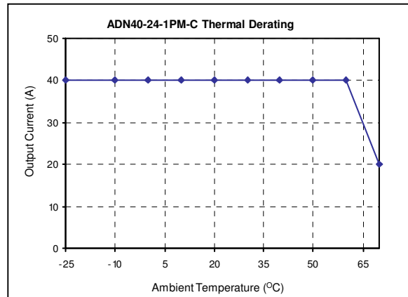
Figure 40: ADN40-24-1PM-C Derating Curve V_{in} = 115V_{ac} I_o = 0 to 40.0A
