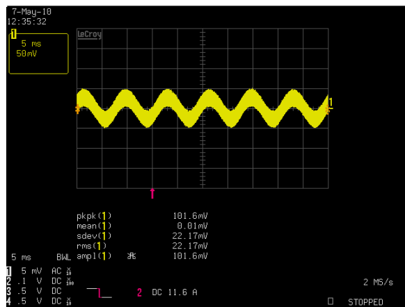
Figure 26: ADN20-24-1PM-C Ripple and Noise Measurement Vin = 115Vac Io = 20.0A Ch 1: Vo
