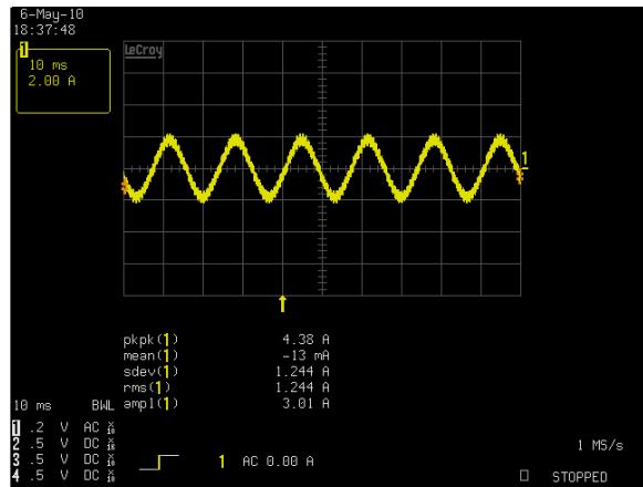
Figure 4: ADN5-24-1PM-C Input Current Waveform Vin = 115Vac Io = 5.0A Ch 1: Io
