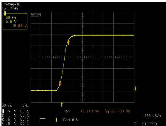
Figure 5: ADN5-24-1PM-C Output Voltage Startup Characteristic Vin = 90Vac Io = 5.0A, Output Capacitance = 330uF/A Ch 1: Vo
