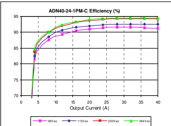
Figure 39: ADN40-24-1PM-C Efficiency Curves @ 25°C, Convection Cool V_{in} = 85 to 264V_{ac} I_o = 0 to 40.0A
