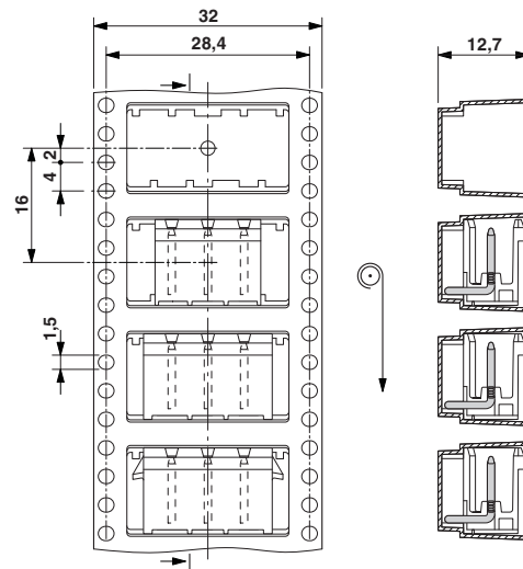
Dimensioned drawing
