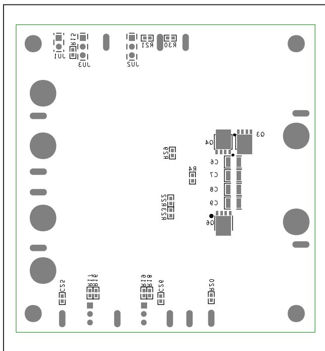
Figure 5. MAX17548 EV Kit Component Placement Guide—Solder Bottom Side
