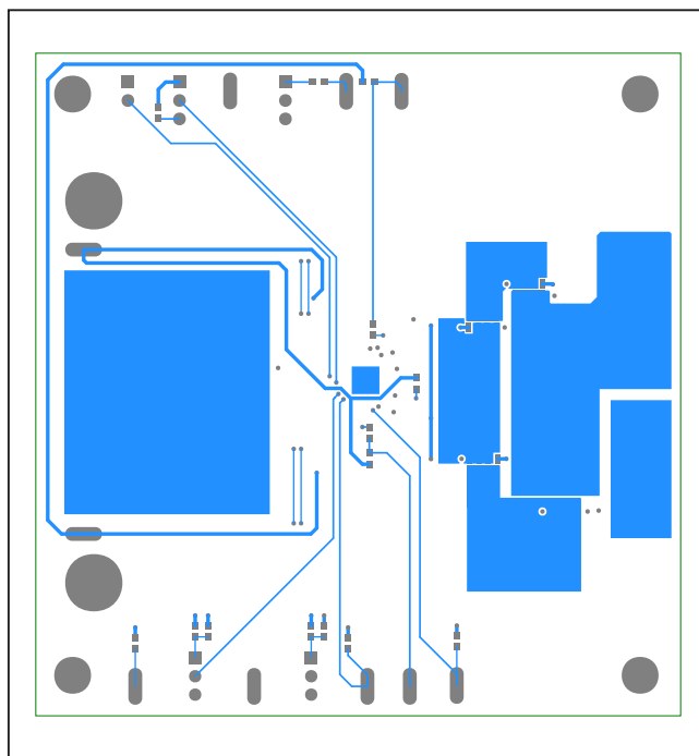
Figure 6. MAX17548 EV Kit PCB Layout—Component Bottom Side
