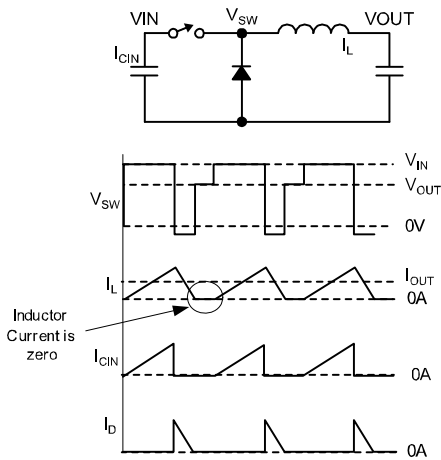
Figure 5. Discontinuous Operation
