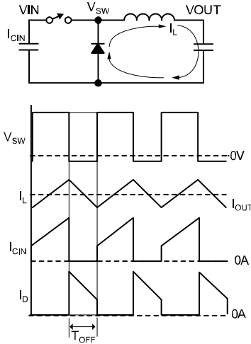
Figure 4. Off-Time
