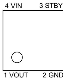
SSON004R1010 (TOP VIEW)
