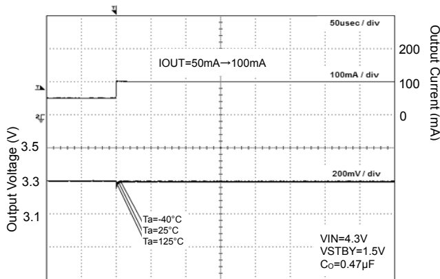
Figure 21. Load Response
