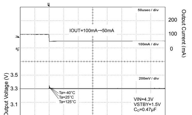
Figure 22. Load Response
