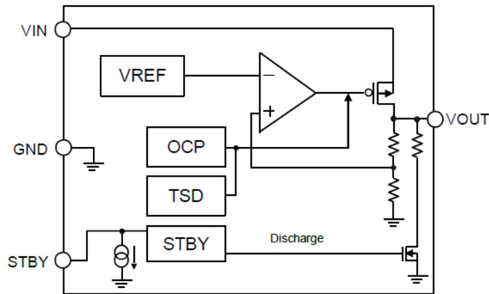
Figure 2. Block Diagram
