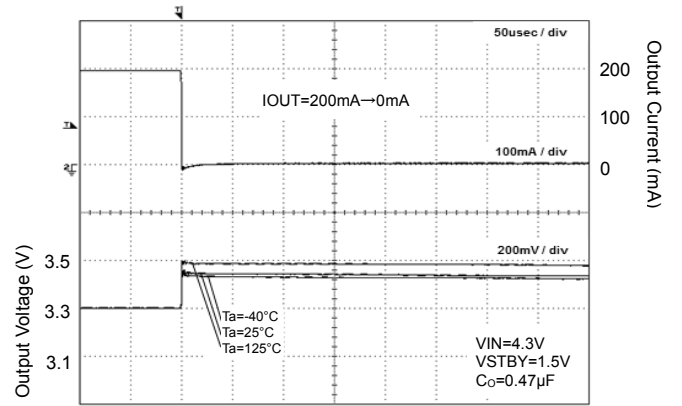
Figure 20. Load Response
