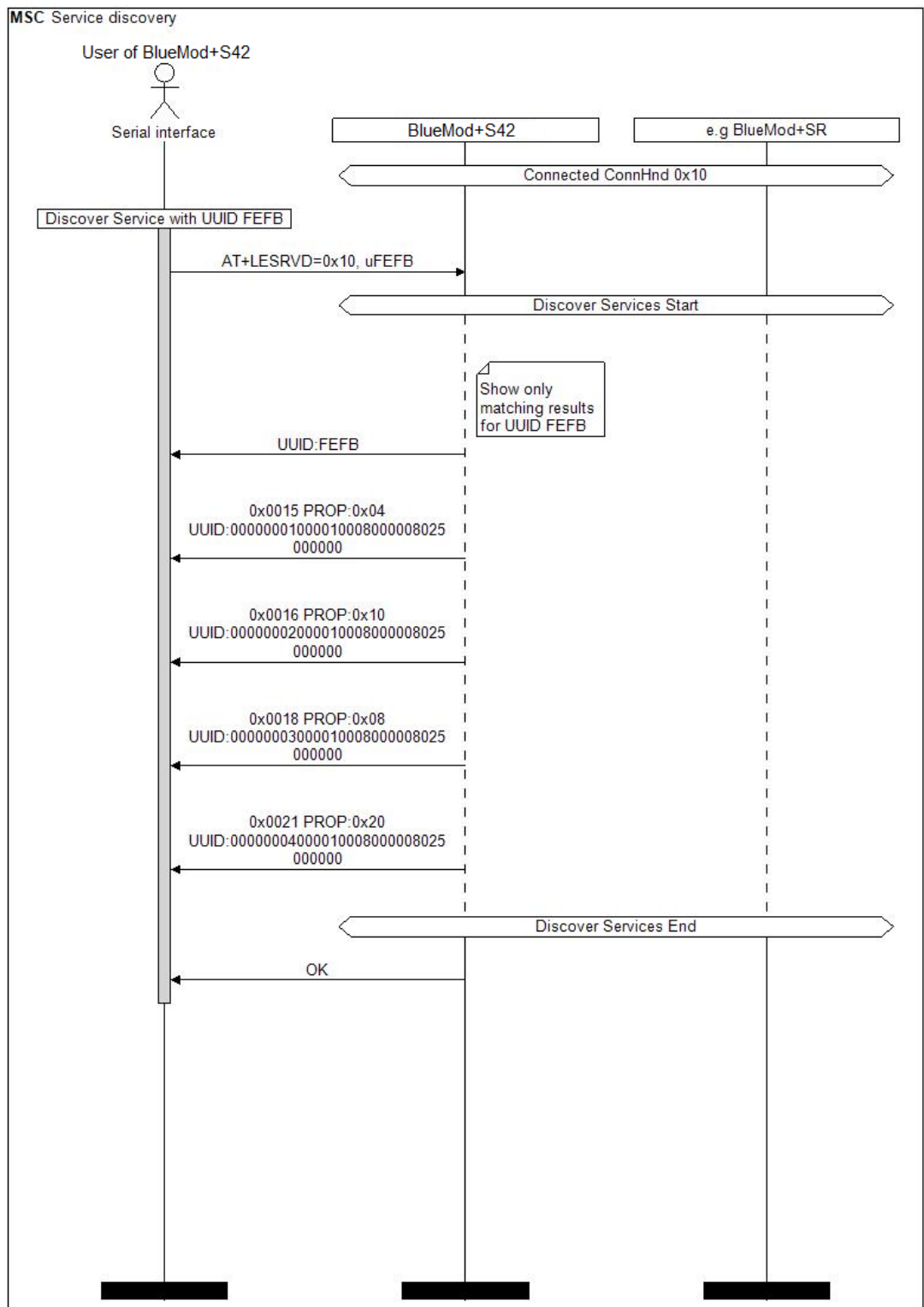
Figure 4: Service discovery
