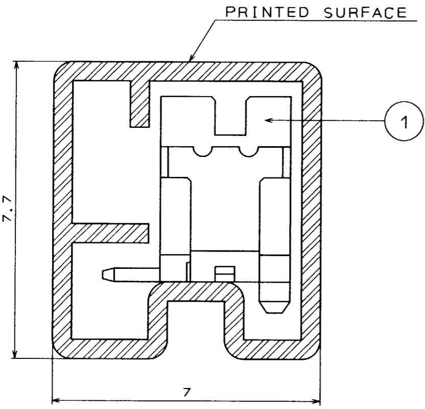
A-A SECTION(10/1)
