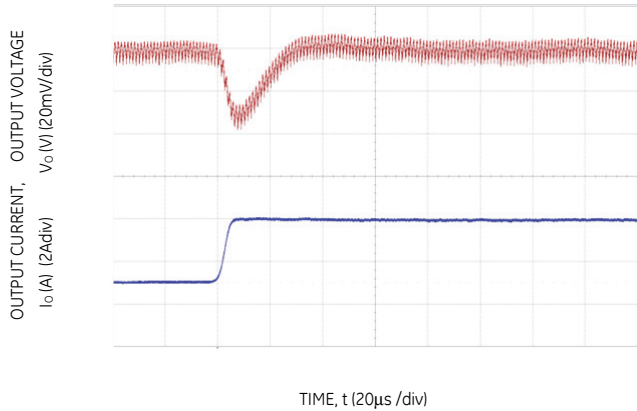
Figure 16. Transient Response to Dynamic Load Change from 50% to 100% at 12Vin, C_{out} = 2 \times 47 \mu F + 1 \times 330 \mu F , C_{Tune} = 2700 pF & R_{Tune} = 300 \Omega
