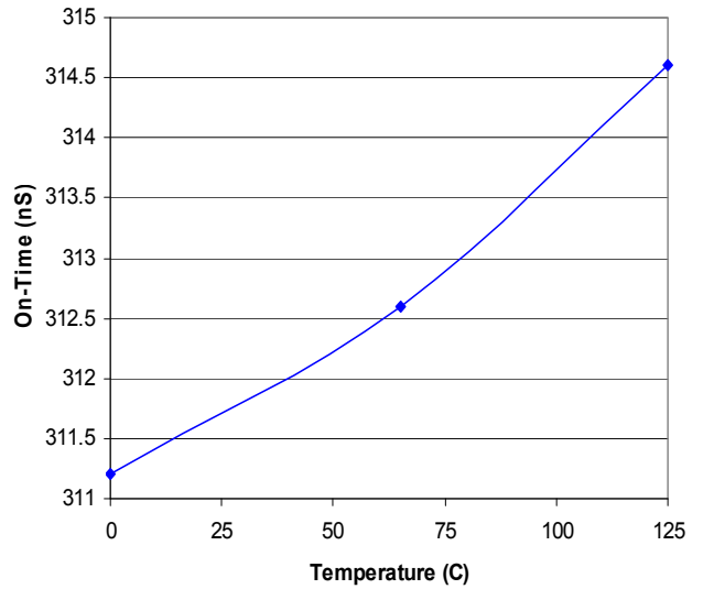
Figure 4. On-Time Variation in CCM: V IN = 12V, V OUT = 1.1V, RFF = 180kOhm
