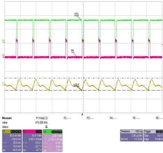
CH1: Vout (50mV/div); CH2: Phase (10V/div) CH4: CPO (2V/div); Time: 2µS/div Figure 13: Charge Pump On at I OUT = 3A
