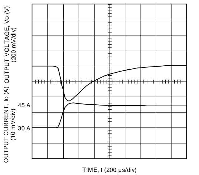
Figure 12. Typical FW300F1 Transient Response to Step Increase in Load from 50% to 75% of Full Load at Room Temperature and 48 V Input (Waveform Averaged to Eliminate Ripple Component.)
