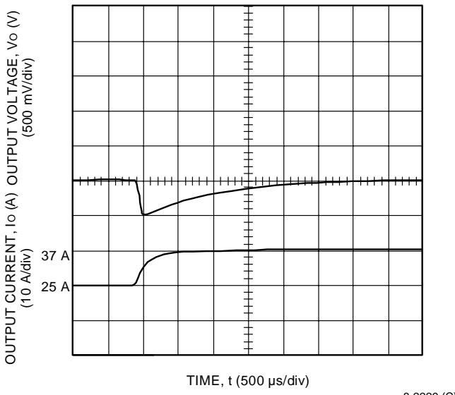
Figure 10. Typical FW250F1 Transient Response to Step Increase in Load from 50% to 75% of Full Load at Room Temperature and 48 V Input (Waveform Averaged to Eliminate Ripple Component.)
