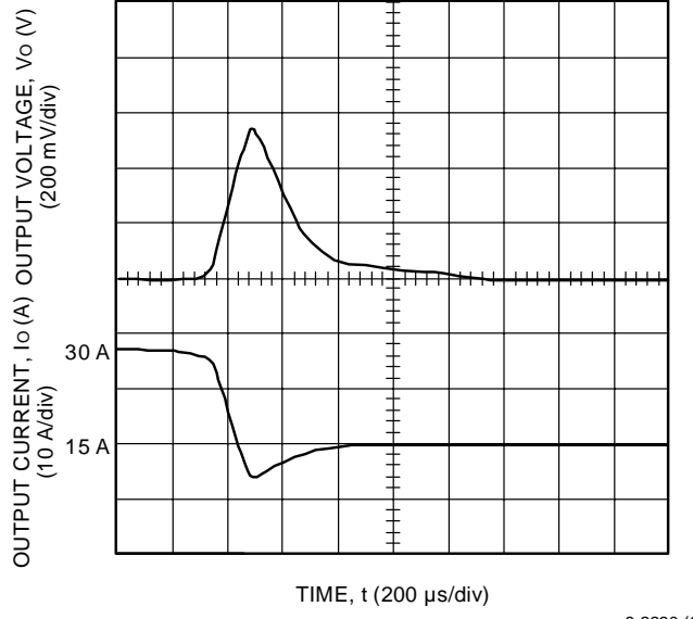
Figure 11. Typical FW300F1 Transient Response to Step Decrease in Load from 50% to 25% of Full Load at Room Temperature and 48 V Input (Waveform Averaged to Eliminate Ripple Component.)
