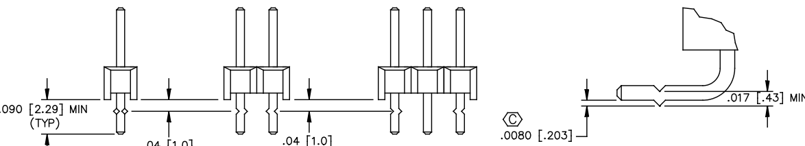
CRIMP DETAIL SCALE: 2x [TYP- ALL CRIMPS]
