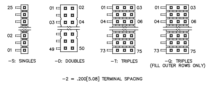
POLARIZATION (STRAIGHT & RA VERSIONS) FIG. 2
