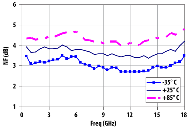
Figure 19. Noise Figure ( V_c = 1.8\text{V} ) over Temp
