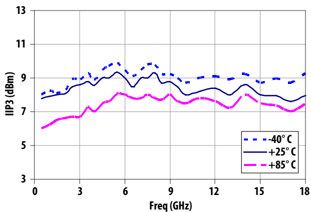
Figure 21. Input IP3 over Temp
