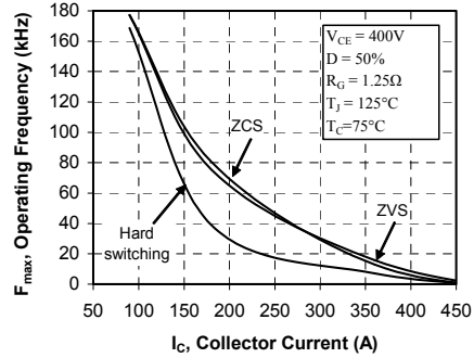
Operating Frequency vs Collector Current
