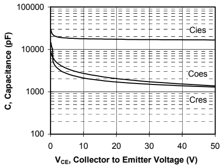
Capacitance vs Collector to Emitter Voltage
