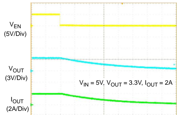
Time (10μs/Div)
