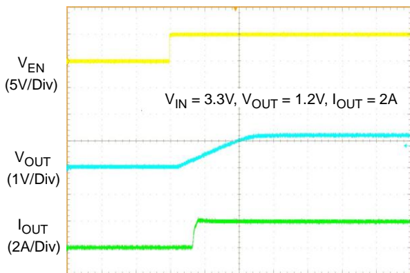
Time (500μs/Div)
