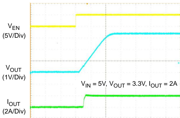
Time (500μs/Div)
