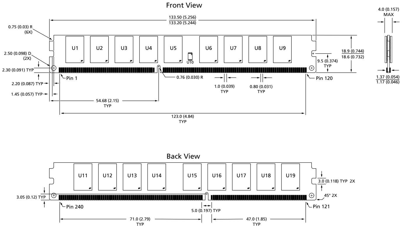
Figure 3: 240-Pin DDR3 VLP UDIMM
