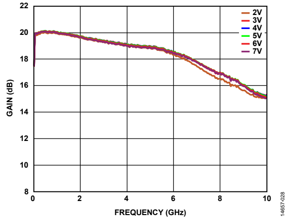
Figure 28. Gain vs. Frequency for Various Supply Voltages, I_{DQ} = 65 mA
