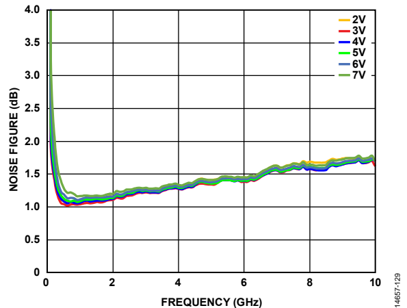
Figure 29. Noise Figure vs. Frequency for Various Supply Voltages, I_{DQ} = 65 mA
