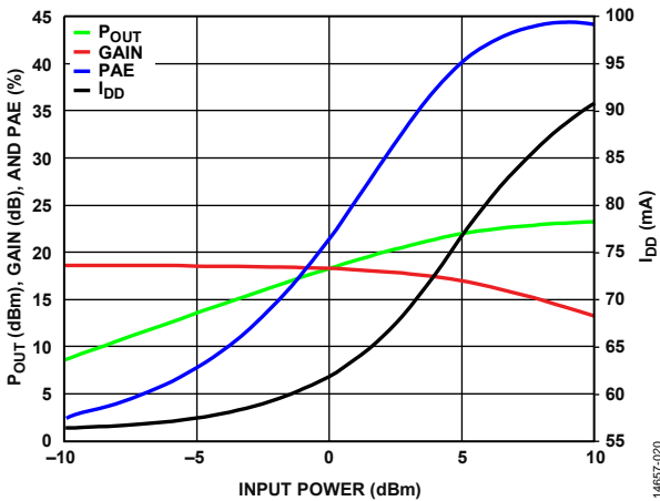
Figure 20. P_{OUT} , Gain, PAE, and Supply Current with RF Applied ( I_{DD} ) vs. Input Power (Performance Below 100 MHz Is Limited by the Bias Network and Does Not Reflect True Device Performance)
