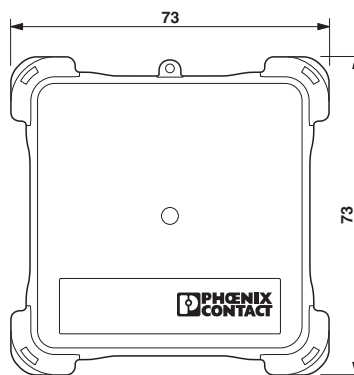
Dimensional drawing
