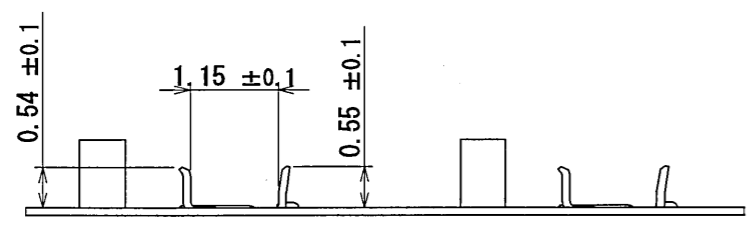
DERECTION B-B SCALE (10:1)
