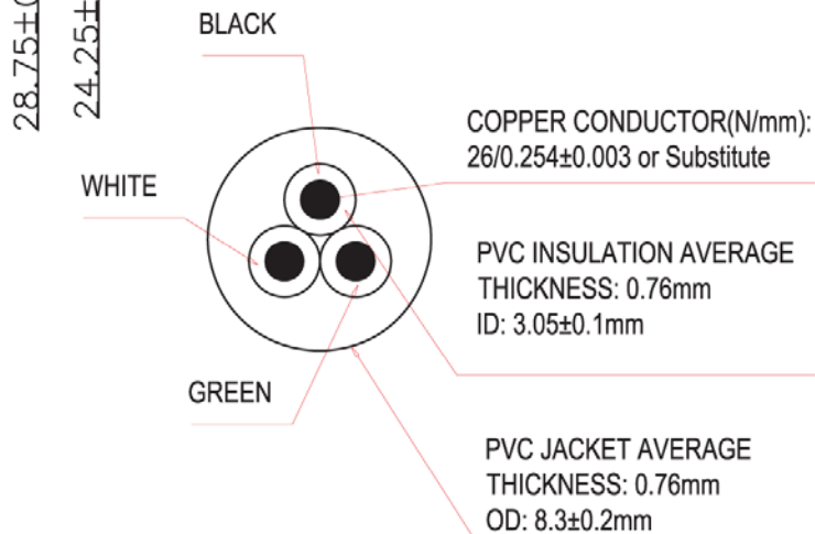
Wire cross section
