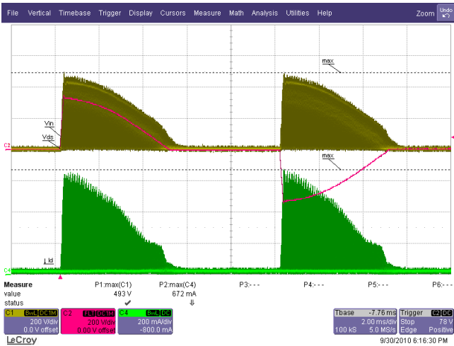
Figure 43 – 230 VAC / 50 Hz, 90° Dimming Phase Angle. 6 LED in Series (18.2 V / 350 mA) Ch1(Yellow): V_{DS} , 200 V / div. Ch2(Red): V_{IN} , 200 V / div. Ch4(Green): I_{DS} , 200 mA / div., 2 ms / div.
