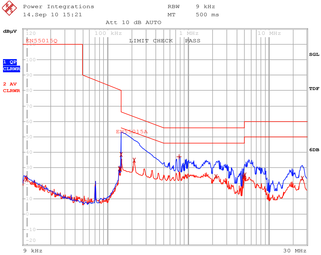
Figure 81 – Pre-scan Conducted EMI, Maximum Steady State Load, 230 VAC, 60 Hz, and EN55015 Limits. Note Blue Line is Peak Result vs. QP Limit Line – Refer to Table for QP Margin.
