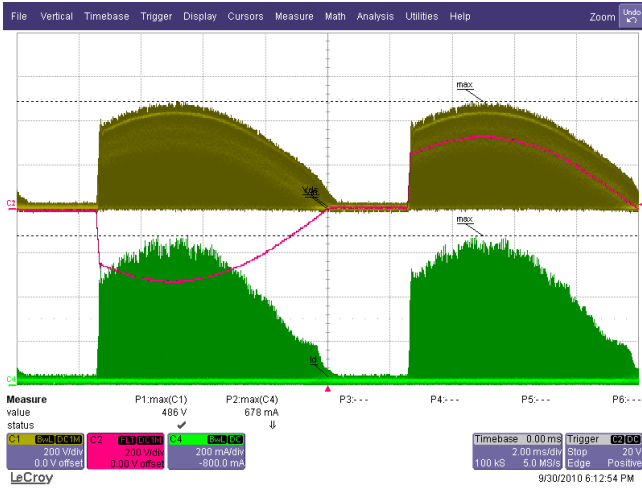
Figure 41 – 230 VAC / 50 Hz, 45° Dimming Phase Angle. 6 LED in Series (18.2 V / 350 mA) Ch1(Yellow): V_{DS} , 200 V / div. Ch2(Red): V_{IN} , 200 V / div. Ch4(Green): I_{DS} , 200 mA / div., 2 ms / div.
