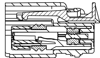
SECTION A-A TPA SHOWN IN FINAL LOCKED POSITION
